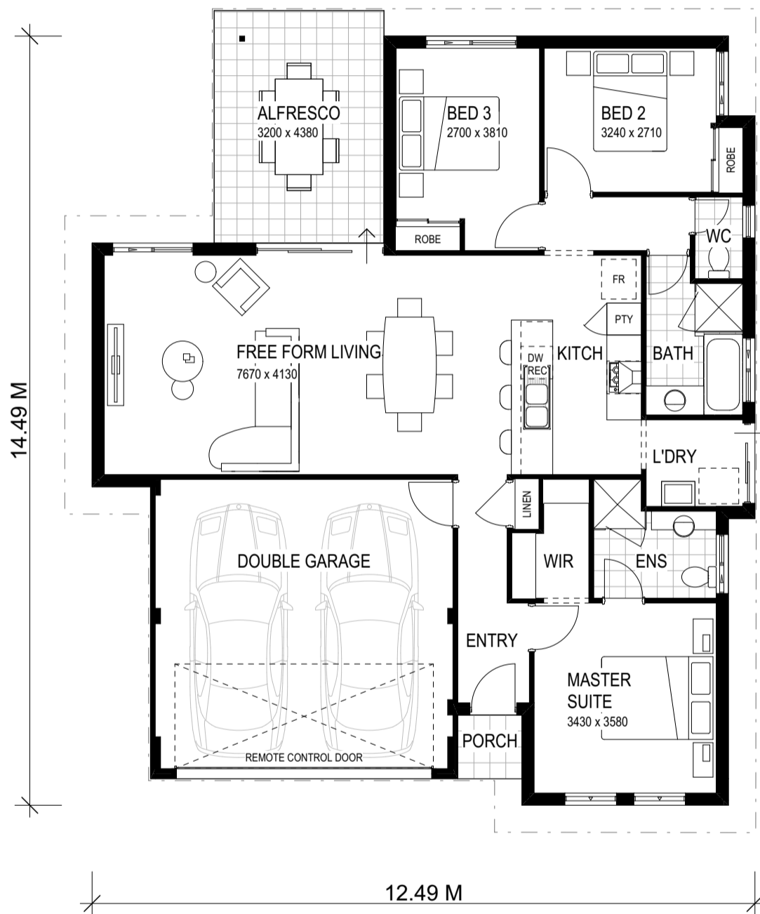
FLOOR PLAN 1:100
