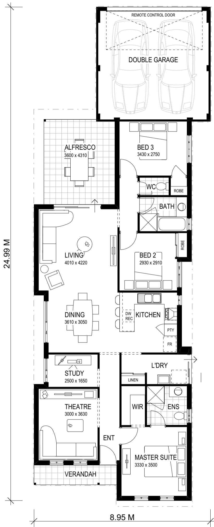
FLOOR PLAN 1:100
